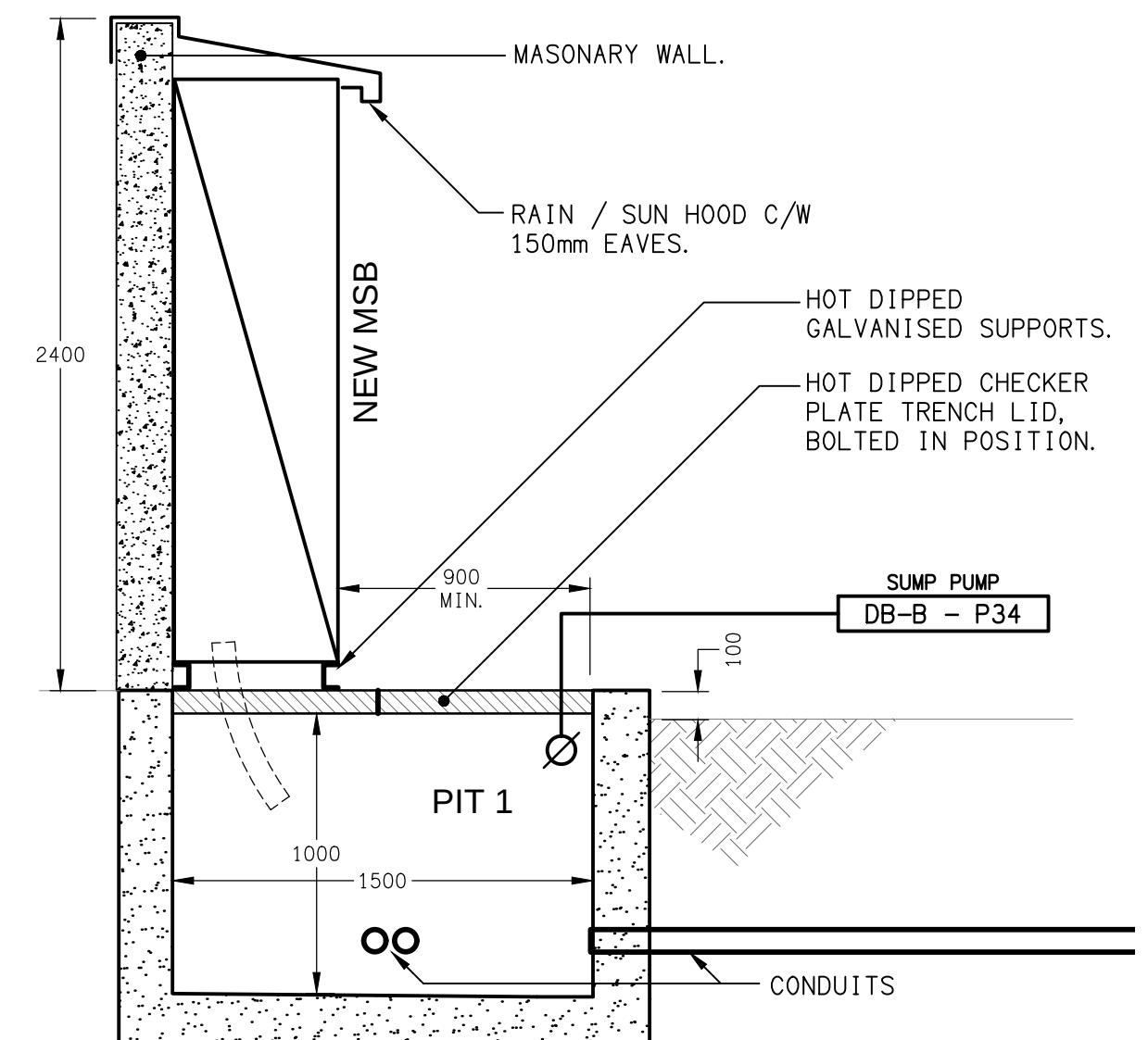
DETAIL A MSB / PIT 1 SECTION VIEW SCALE 1:25
